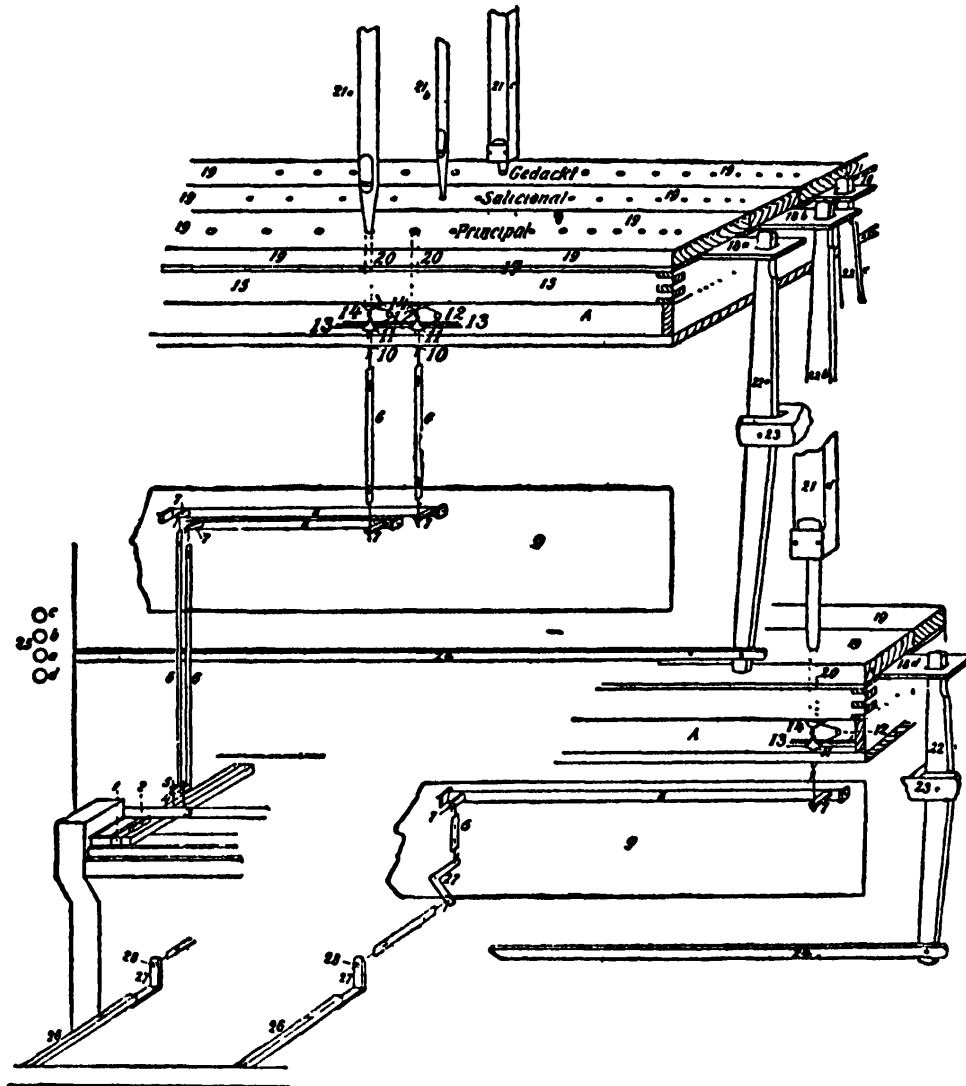
FIGURE 158. Section of a mechanical organ. After H. Schmidt.
